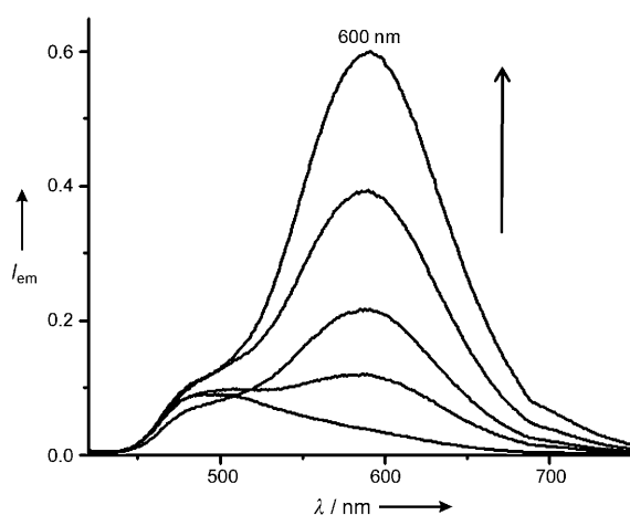
Figure 3. a) Increase in the emission intensity of S q1 ( 6 \times 10^{-6} M) at 600 nm ( \lambda_{\text{ex}} = 410 nm) upon addition of aliquots (0, 20, 30, 40 \mu L) of human blood plasma after reduction.
